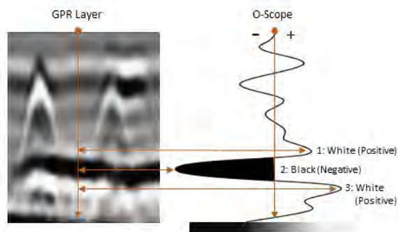
The first reflector is white (positive), but the first-biggest-brightest reflector is black (negative). This demonstrates that the GPR energy accelerated at the concrete/layer contact. This target could be interpreted as an air-filled void at the base of the slab.
