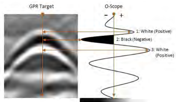
The first reflector is white (positive), but the first-biggest-brightest reflector is black (negative). This demonstrates that the GPR energy accelerated at the concrete/target contact. This target could be interpreted as air-filled PVC or potentially as a small air void.
