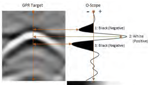
The first reflector is black (negative), but the first-biggest-brightest reflector is white (positive). This demonstrates that the GPR energy decelerated at the concrete/target contact. This target could be interpreted as metallic or possibly water-filled PVC.
